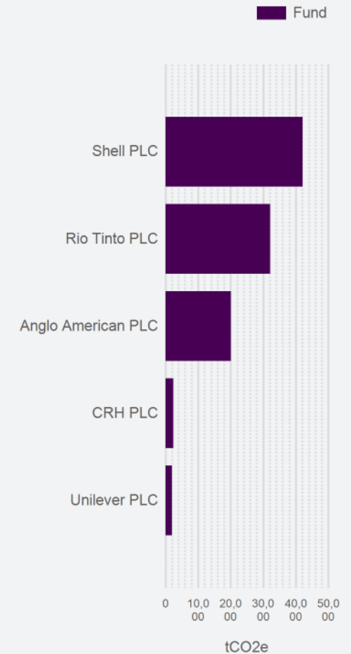
Top fund contributors to Total GHG Emissions (scope 1, 2 and 3)
