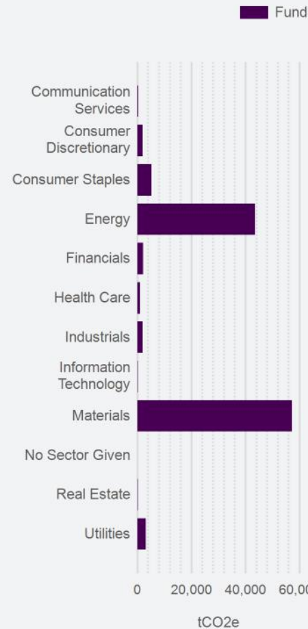
Total GHG Emissions (scope 1, 2 and 3) by sector
